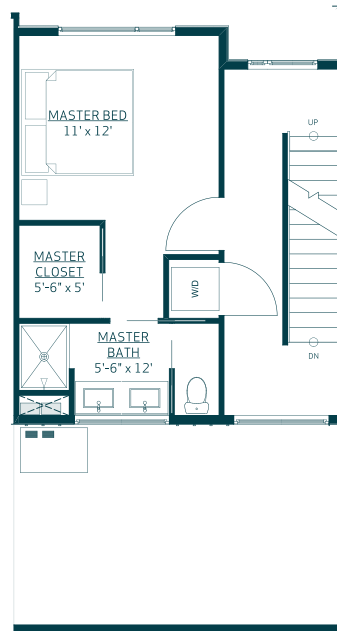
LEVEL 03
