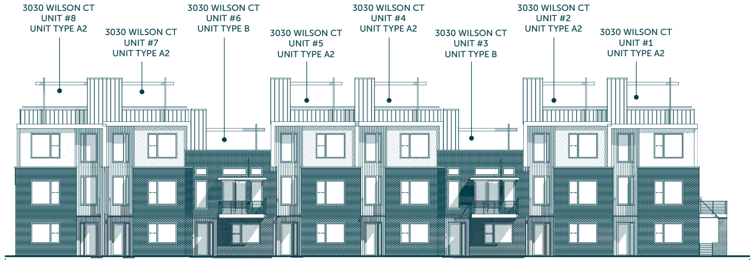
BUILDING 3030
